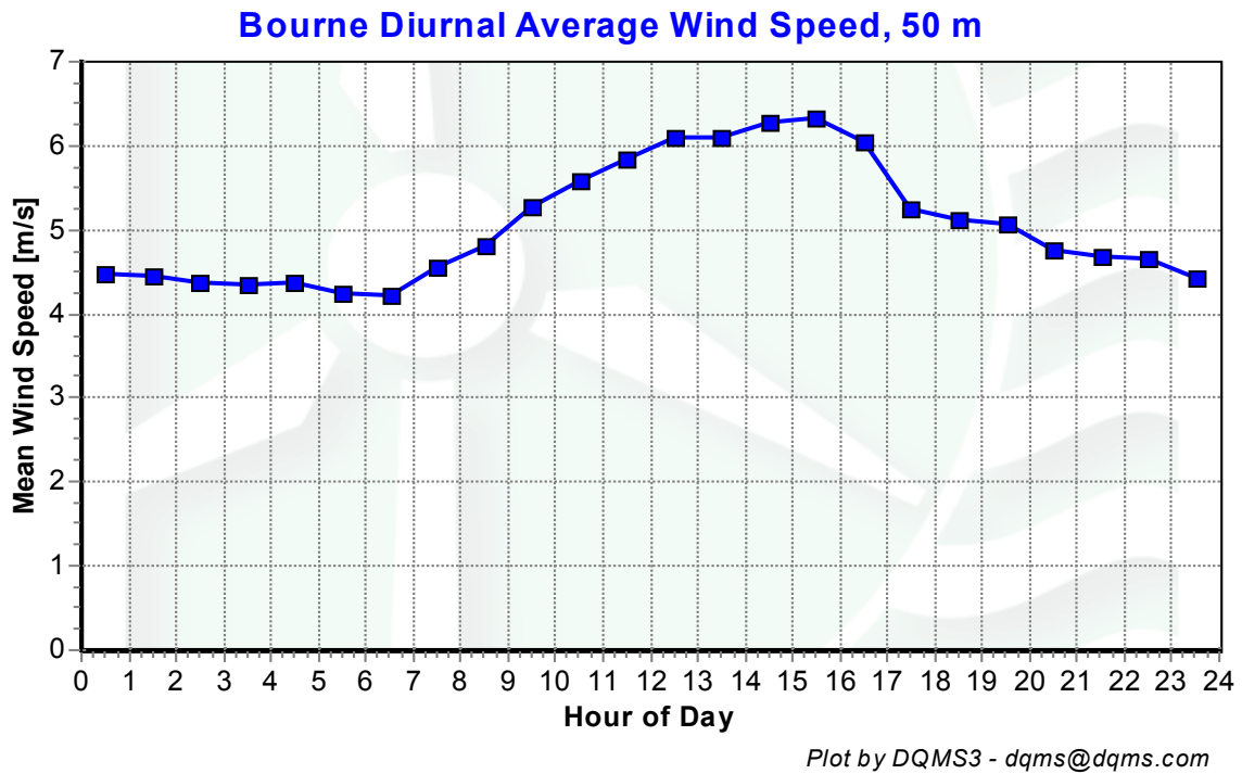
Figure 4 - Diurnal Average Wind Speed, August 2004
