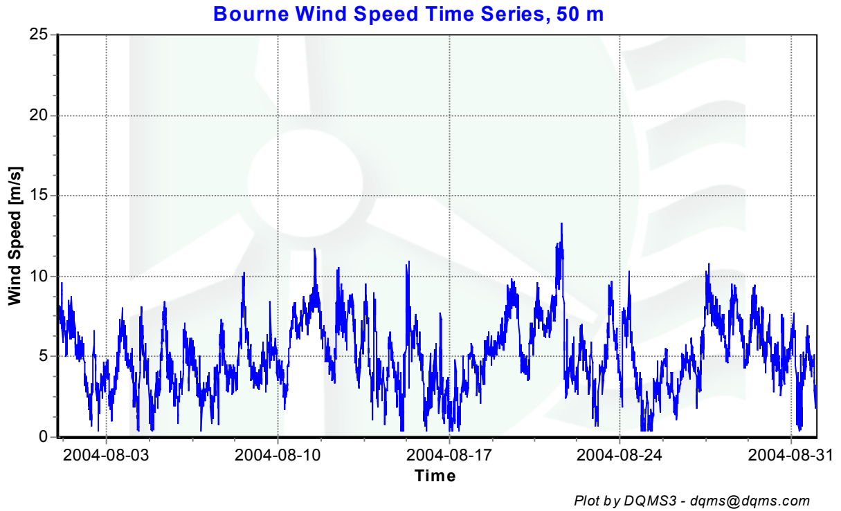
Figure 2 - Wind Speed Time Series, August 2004
