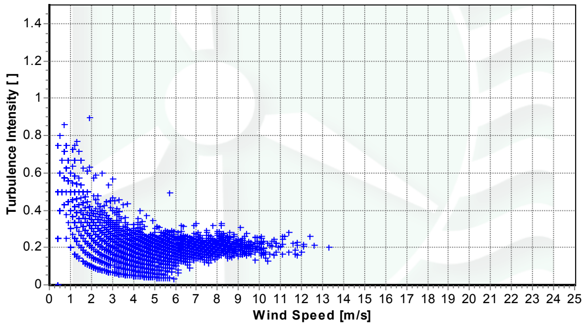
Figure 5 - Turbulence Intensity vs Wind Speed, August 2004
