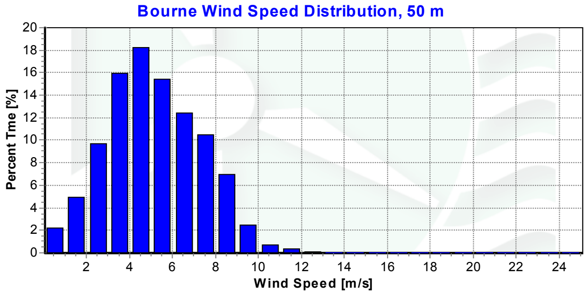
Figure 3 - Wind Speed Distribution, August 2004
