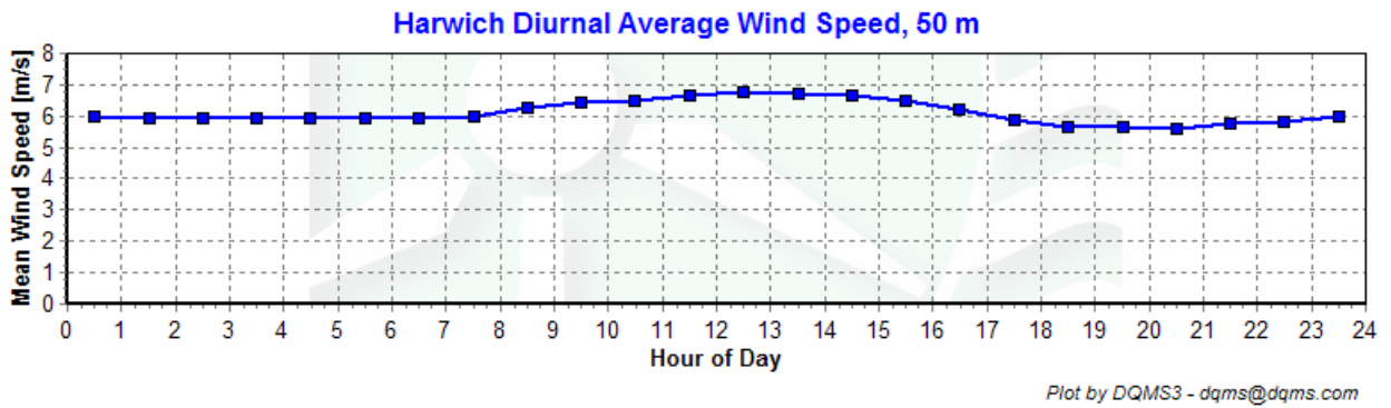
Figure 5 – Diurnal Wind Speed, March 2007 – May 2007
