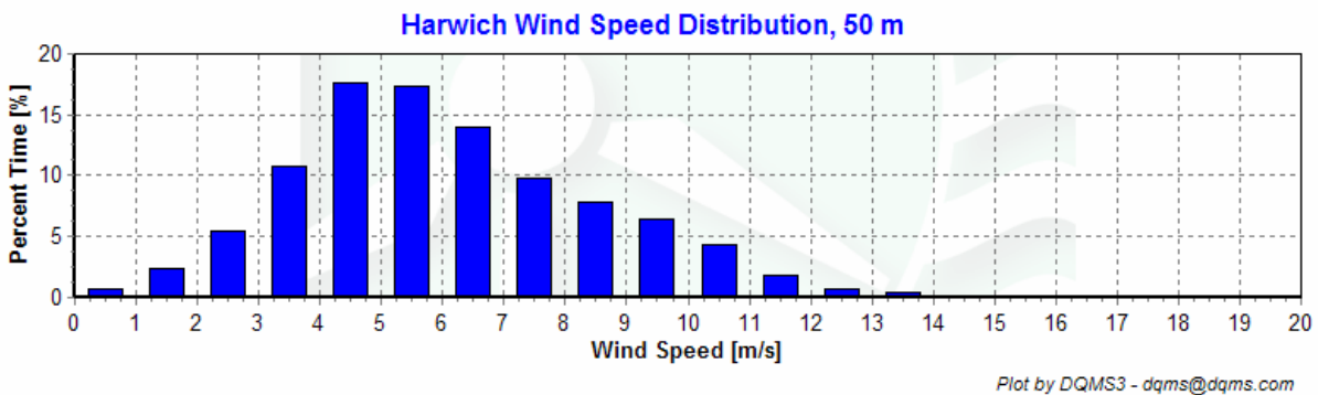
Figure 3 – Wind Speed Distribution, March 2007 – May 2007
