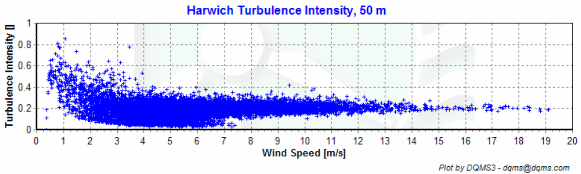
Figure 6 – Turbulence Intensity vs. Wind Speed, March 2007 – May 2007
