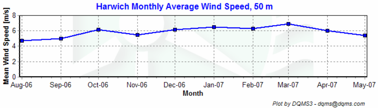
Figure 4 – Monthly Average Wind Speeds, August 2006 – May 2007
