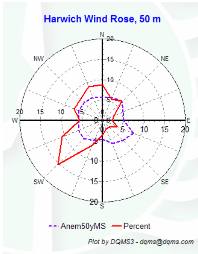
Figure 7 – Wind Rose, March 2007 – May 2007
