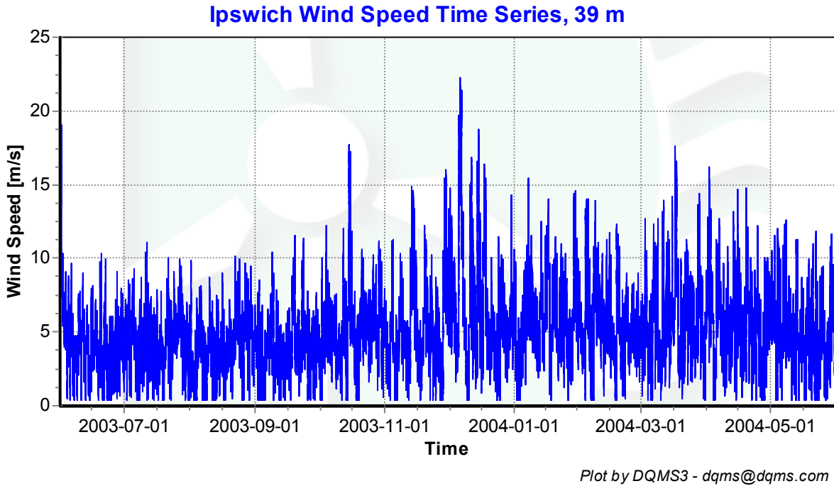
Figure 1 – Wind Speed Time Series, June 2003 – May 2004
