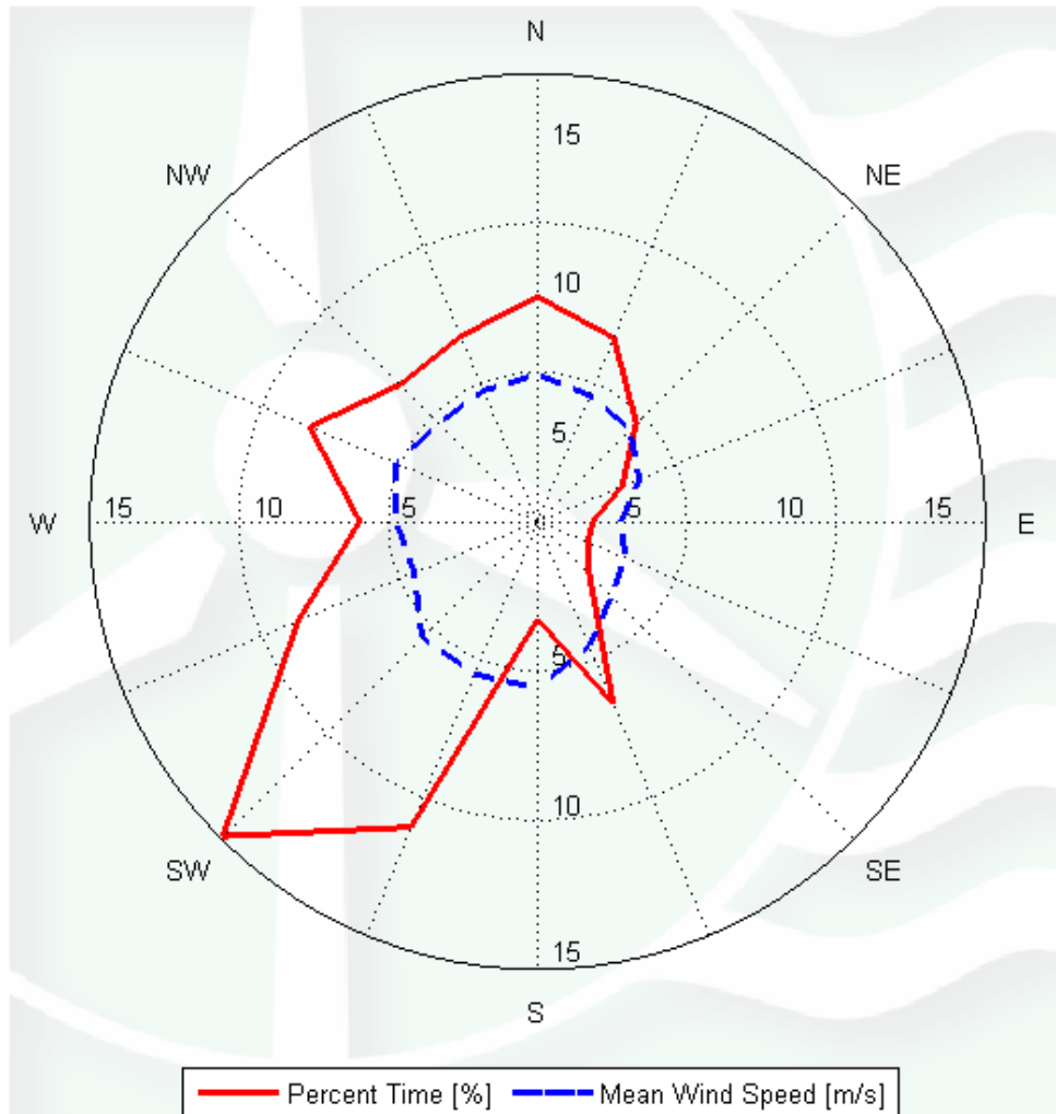
ORR Wind Rose, 49 m
