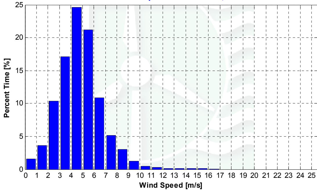
Figure 4 - Wind Speed Distribution, September 1 st 2007—November 30 th 2007
