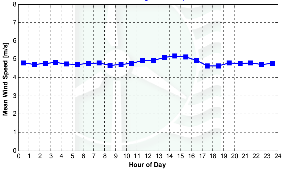
Figure 6 - Diurnal Average Wind Speed, September 1 st 2007—November 30 th 2007
