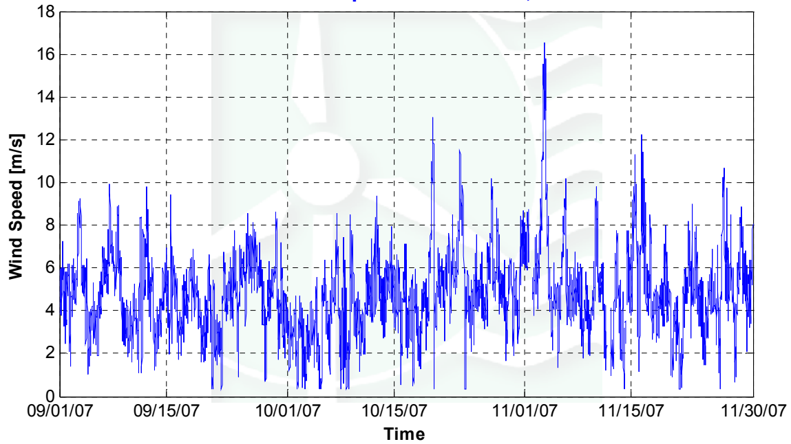
Figure 3 - Wind Speed Time Series, September 1 st 2007—November 30 th 2007
