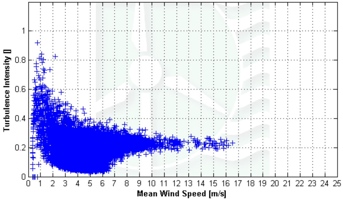
Figure 7 - Turbulence Intensity, September 1 st 2007—November 30 th 2007
