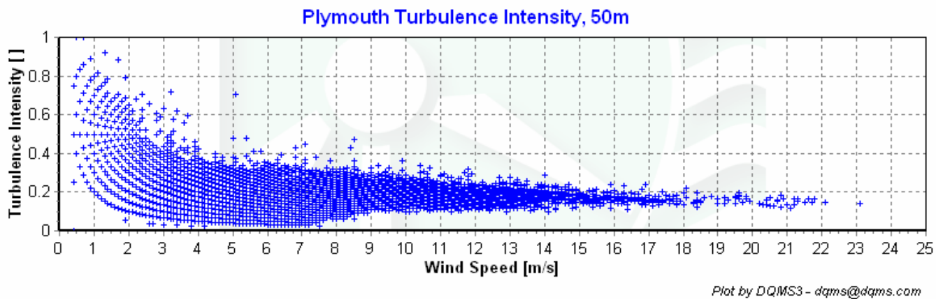
Figure 6 – Turbulence Intensity vs. Wind Speed, June 2007 – May 2008
