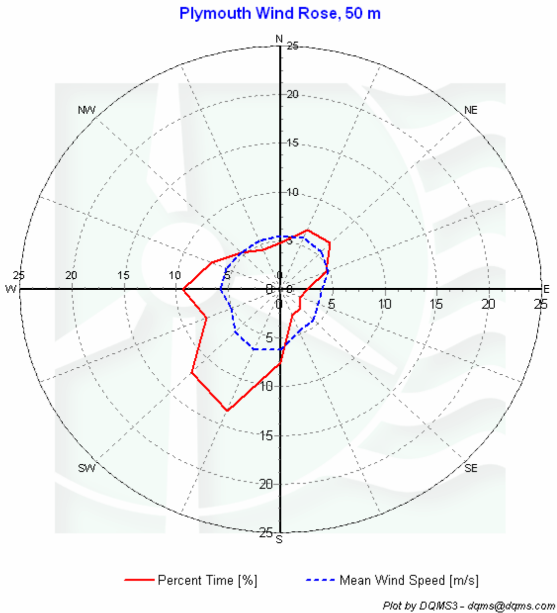
Figure 7 – Wind Rose, June 2007 – May 2008
