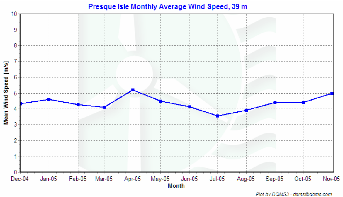
Figure 5 -- Monthly Average Wind Speed, December 1, 2004– December 1, 2005
