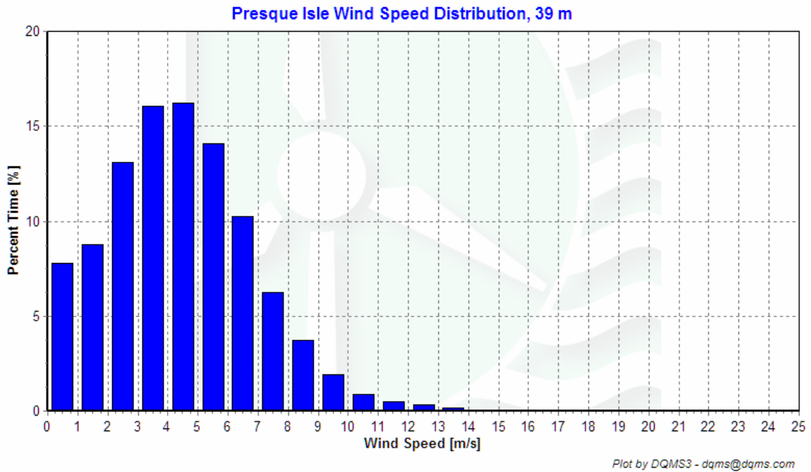
Figure 4 – Wind Speed Distribution, December 1, 2004 – December 1, 2005
