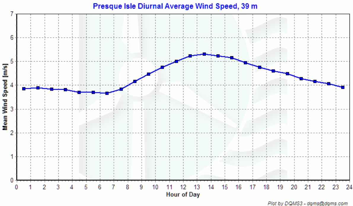
Figure 6 – Diurnal Wind Speed, December 1, 2004 – December 1, 2005
