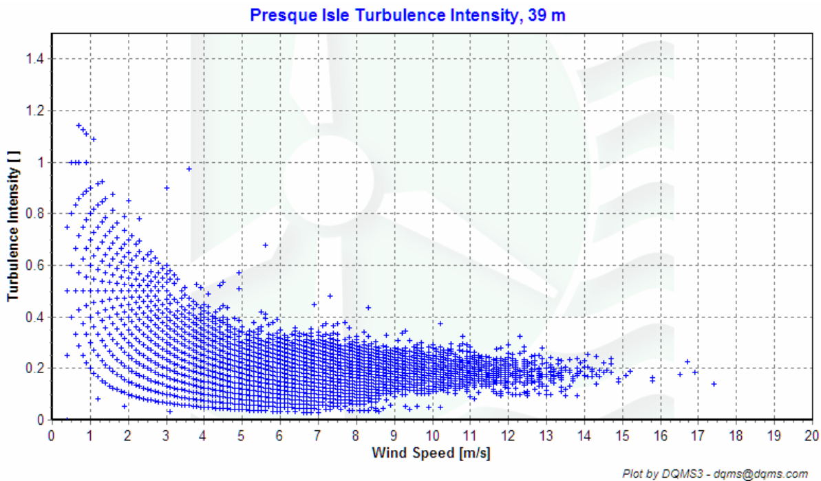
Figure 7 – Turbulence Intensity vs Wind Speed, December 1, 2004 – December 1, 2005
