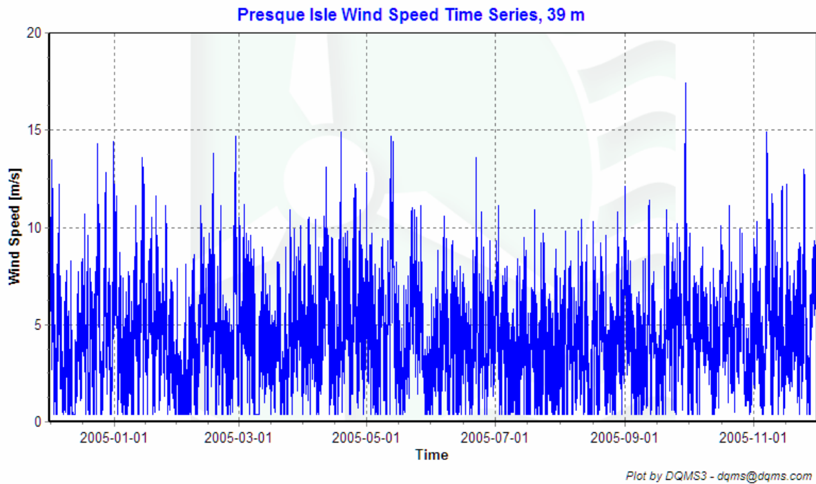
Figure 3 – Wind Speed Time Series, December 1, 2004 – December 1, 2005
