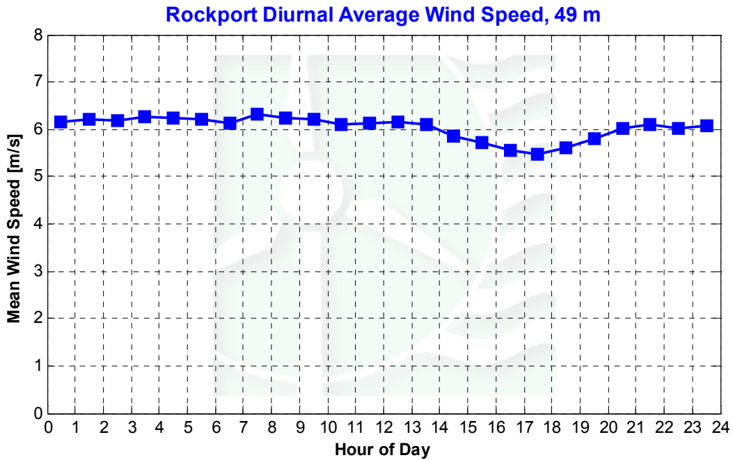
Figure 6 - Diurnal Average Wind Speed, December 1 st 2007 -- February 29 th 2008
