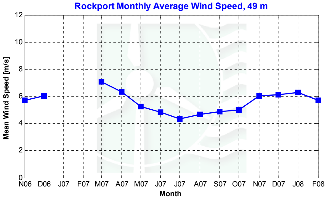
Figure 5 - Monthly Average Wind Speed
