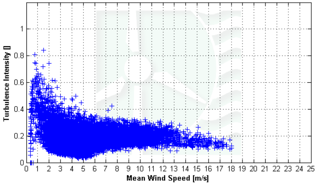
Figure 7 - Turbulence Intensity, December 1 st 2007 -- February 29 th 2008
