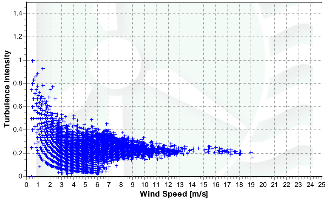
Figure 6 - Turbulence Intensity, September 1 st 2007—November 30 th 2007
