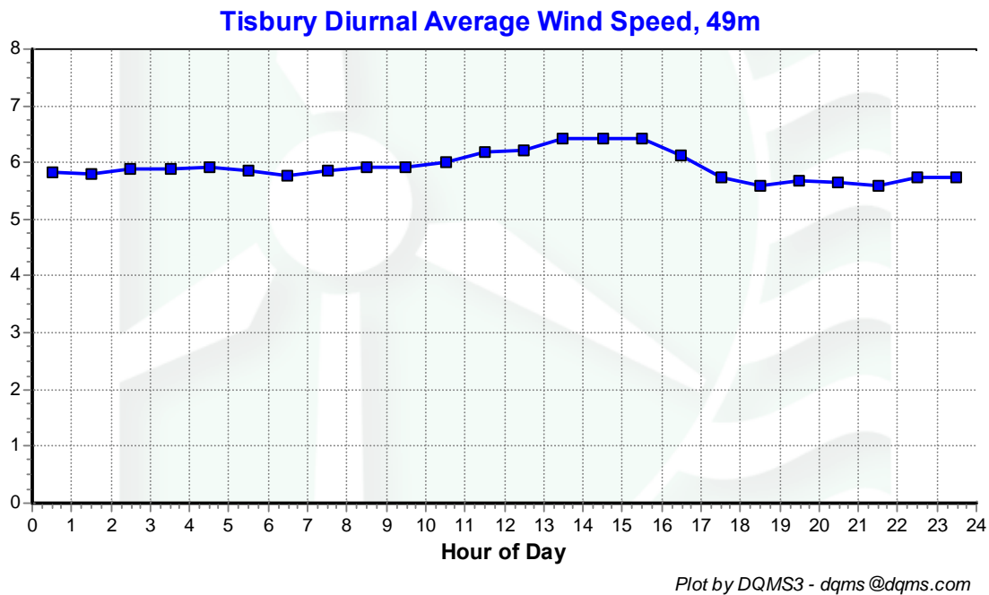
Figure 5 - Diurnal Average Wind Speed, March 1 st 2008 – May 31 st 2008
