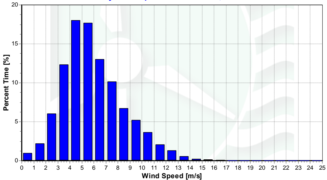
Figure 3 - Wind Speed Distribution, March 1 st 2008 – May 31 st 2008
