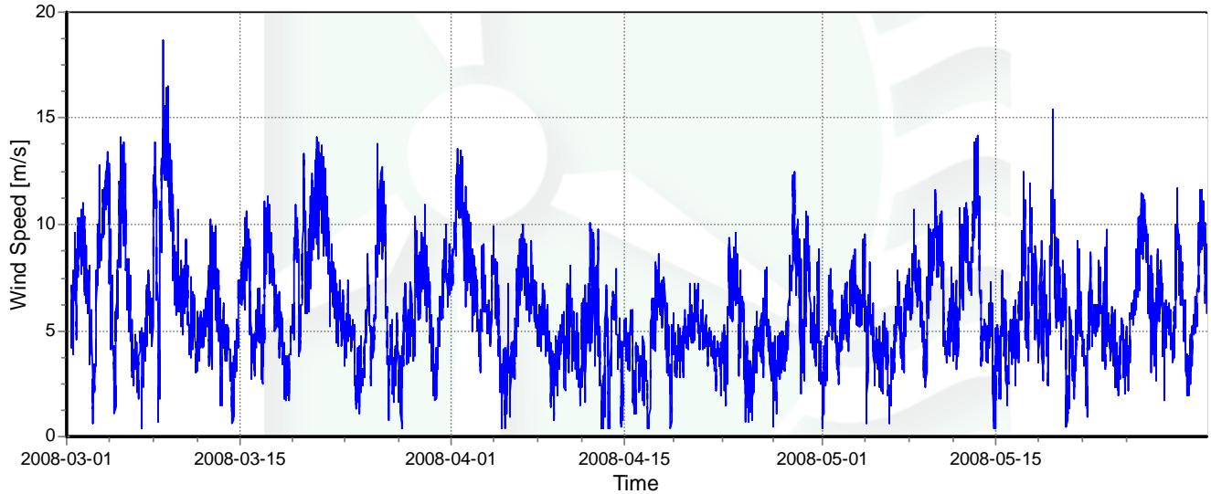
Figure 2 - Wind Speed Time Series, March 1 st 2008 – May 31 st 2008
