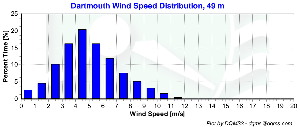
Figure 2 – Wind Speed Distribution, March 1, 2009 – May 31, 2009
