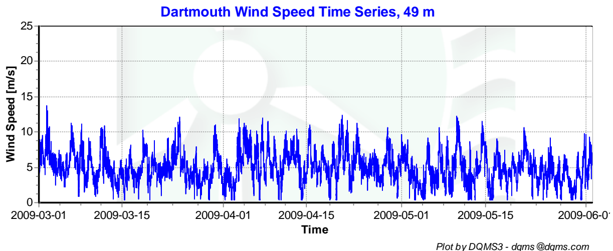
Figure 2 – Wind Speed Time Series, March 1, 2009 – May 31, 2009
