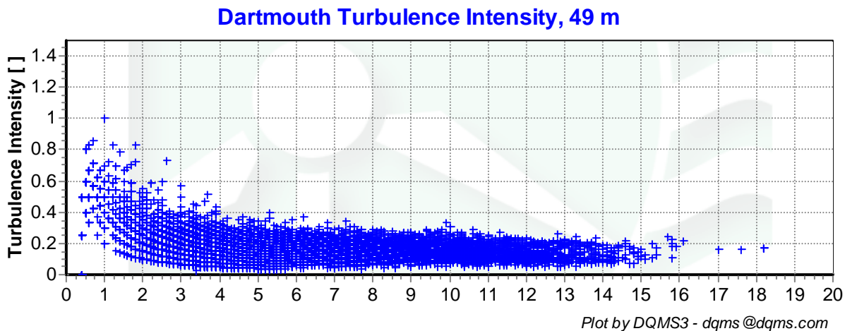
Figure 5 – Turbulence Intensity vs. Wind Speed, March 1, 2009 – May 31, 2009
