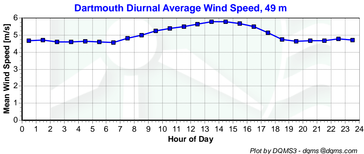
Figure 4 – Diurnal Average Wind Speeds, March 1, 2009 – May 31, 2009
