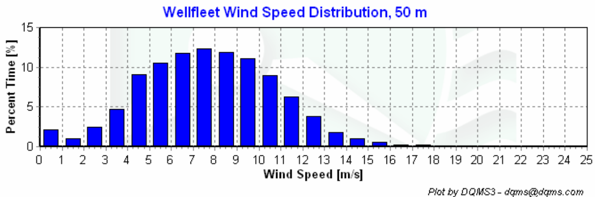
Figure 3 - Wind Speed Distribution, December 1, 2006 – February 28, 2007
