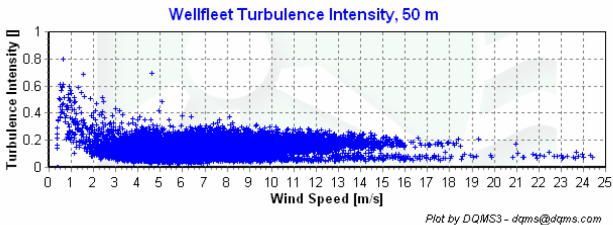
Figure 6 – Turbulence Intensity, December 1, 2006 – February 28, 2007.
