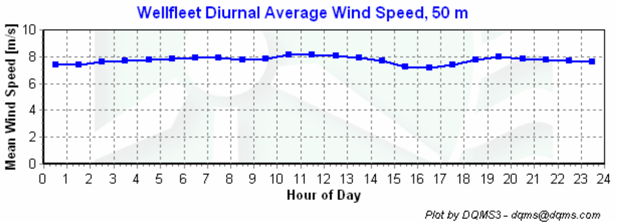
Figure 5 - Diurnal Average Wind Speed, December 1, 2006 – February 28, 2007
