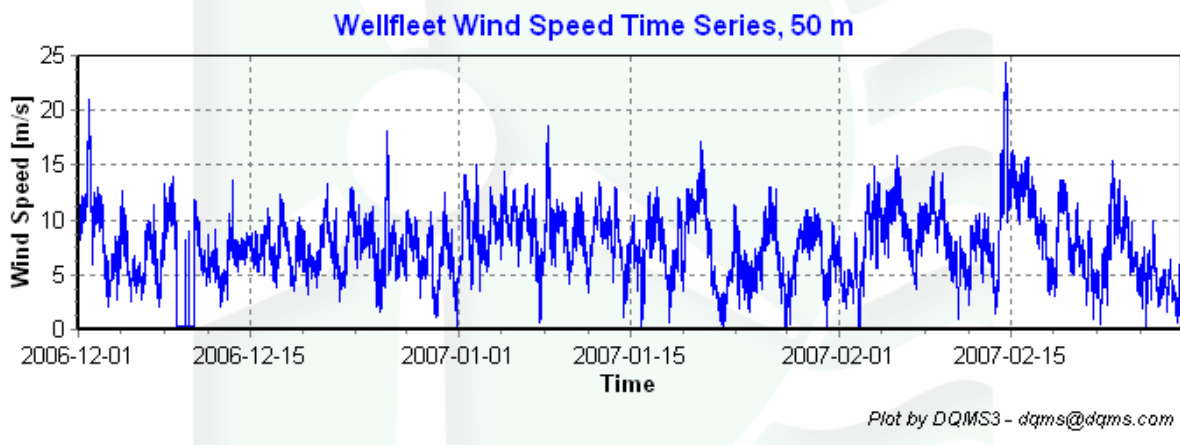
Figure 2 - Wind Speed Time Series, December 1, 2006 – February 28, 2007
